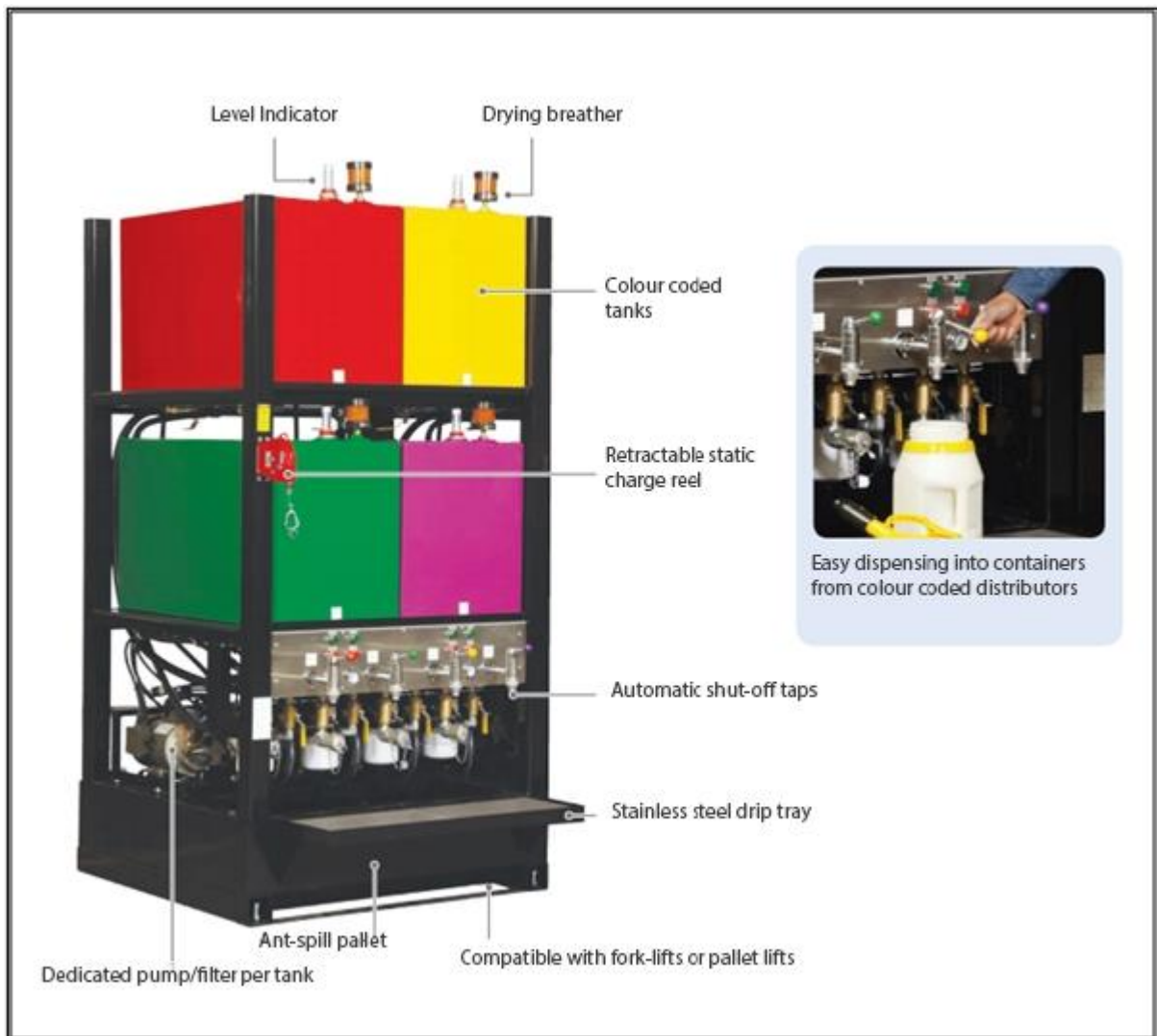
Example of a storage station from SKF
